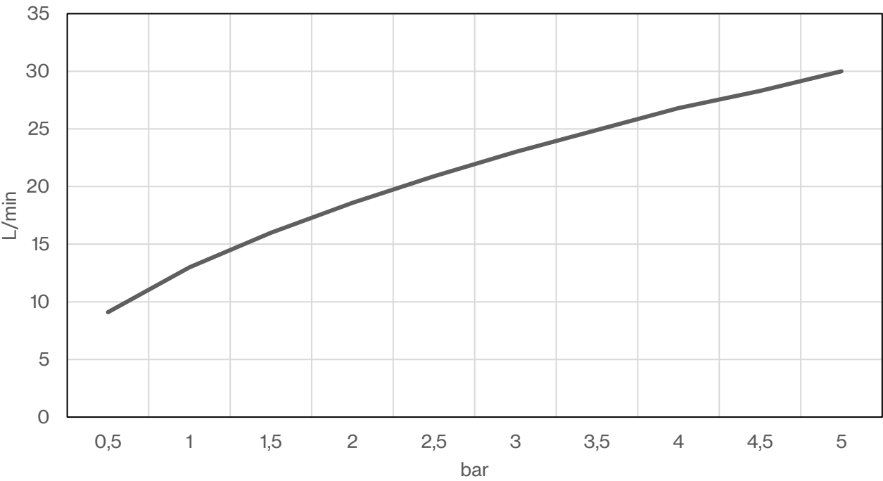
QT3100 built-in part only (flowrate L/min)
