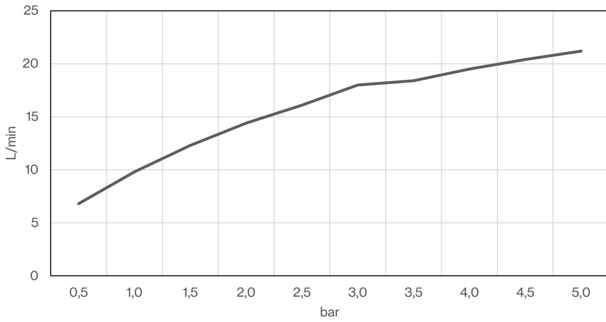
QA3290 flow rate (without aerator)
