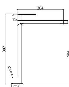
TA 081-085CR Miscelatore lavabo prolungato con/ senza scarico Tall wash basin mixer with/without pop up waste
