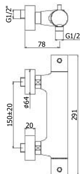
LIQ 168-168DCR Miscelatore termostatico doccia attacco 1/2" con/ senza set doccia Thermostatic shower mixer 1/2" connection with/ without shower kit
