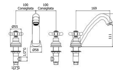
IRV 052-055 Batteria lavabo con canna fissa con/senza scarico Three-hole wash basin mixer with fixed spout with/without pop up waste
