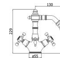
FBLV 131-135CR Monoforo bidet con/senza scarico One-hole bidet mixer with/without pop up waste
