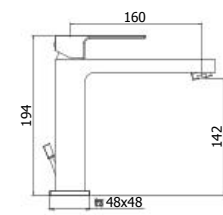
EL 074-073CR Miscelatore lavabo medio con/ senza scarico Medium wash basin mixer with/ without pop up waste
