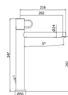
JK 081-085CR Miscelatore lavabo prolungato con/ senza scarico Tall wash basin mixer with/ without pop up waste
