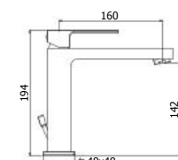
EF 074-073CR Miscelatore lavabo medio con/ senza scarico Medium wash basin mixer with/ without pop up waste
