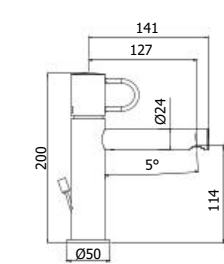
JK 071-075CR Miscelatore lavabo con/ senza scarico Wash basin mixer with/ without pop up waste
