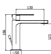
TA 071-075CR Miscelatore lavabo con/senza scarico Wash basin mixer with/without pop up waste
