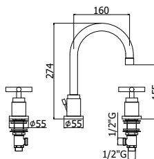
QTV 052-055 Batteria lavabo con/senza scarico Three-hole wash basin mixer with/without pop up waste
