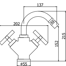
QTV 138-137CR Monoforo bidet con/senza scarico One-hole bidet mixer with/without pop up waste
