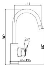
BR 078-077CR Miscelatore lavabo canna tonda orientabile con/senza scarico Wash basin mixer round swivel spout with/without pop up waste
