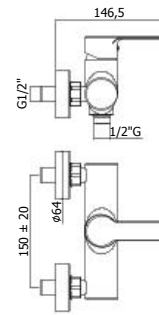
RED 168-168DCR Miscelatore doccia con/senza set doccia Wall mounted shower mixer with/without shower set
