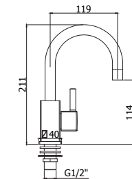
LEA 091 Rubinetto lavabo canna orientabile, con vitone ceramico Basin tap with swivelling spout and ceramic disk valve
