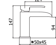
LES 061-065CR Miscelatore lavabo a cascata con/senza scarico Waterfall basin mixer with/without pop up waste
