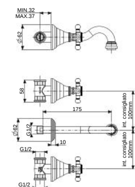
FBLV 003-008CR Batteria lavabo incasso con bocca a muro 175 / 245 mm Three-hole concealed wash basin mixer with wall spout 175 / 245 mm
