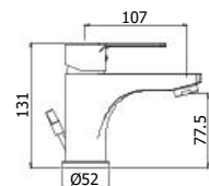
RED 071-075CR-EWS Con cartuccia ENERGY & WATER SAVING With ENERGY & WATER SAVING cartridge
