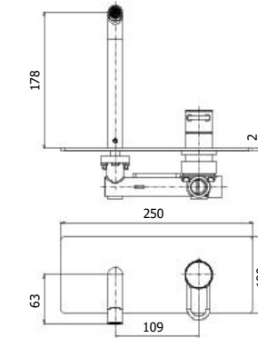
JK 105-104-106CR Miscelatore incasso con bocca erogazione a muro 178 mm / 123 mm / 248 mm Concealed wash basin mixer with wall spout 178 mm / 123 mm / 248 mm
