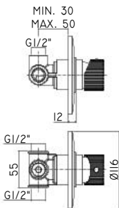
JO 010-011CR Miscelatore incasso doccia / Piastra Ø116 e 110 mm Concealed shower mixer / Wall plate Ø116 and 110 mm
