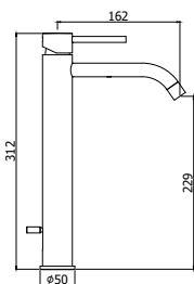
LIG 081-085CR Miscelatore lavabo prolungato con/senza scarico Tall wash basin mixer with/without pop up waste
