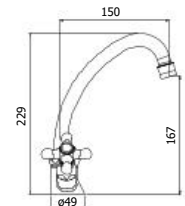
IRV 078-077CR Monoforo lavabo con bocca orientabile con/senza scarico One-hole wash basin mixer with swivelling spout with/without pop up waste
