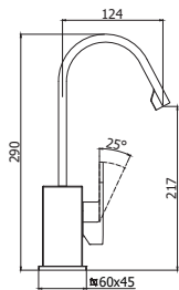
EF 878-877CR Miscelatore lavabo canna piatta orientabile con/senza scarico Wash basin mixer with rectangular swivel spout with/without pop up waste
