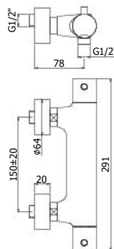
LIQ 168E-168EDCR Miscelatore termostatico doccia attacco 1/2" con/ senza set doccia, con limitatore di portata ECO-STOP Thermostatic shower mixer 1/2" connection with/ without shower kit, with flow reducer ECO-STOP
