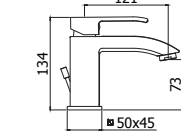
LES 071-075CR Miscelatore lavabo con/senza scarico Wash basin mixer with/without pop up waste
