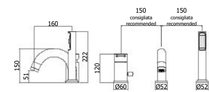
JK 047-048CR MAX FLOW Miscelatore bordo vasca con doccia estraibile, con/ senza bocca erogazione Deck mounted bath mixer with pull out hand-shower, with/ without spout
