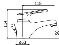
NT 071-075CR Miscelatore lavabo con/senza scarico Wash basin mixer with/without pop up waste
