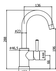
BI 078-077CR Miscelatore lavabo con canna orientabile con/senza scarico Wash basin mixer with swivelling spout with/without pop up waste
