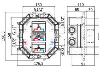
CPBOX 001 Set incasso universale per miscelatori e termostatici compact (1, 2 o 3 uscite) Universal concealed set for compact mixers and thermostatic mixers (1, 2 or 3 outlets)
