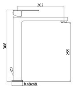
EL 081-085CR Miscelatore lavabo prolungato con/ senza scarico Tall wash basin mixer with/ without pop up waste
