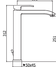
LES 081-085CR Miscelatore lavabo prolungato, con/senza scarico Tall wash basin mixer with/without pop up waste
