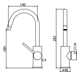
LIG 078-077CR Miscelatore lavabo con canna orientabile con/senza scarico Wash basin mixer with swivelling spout with/without pop up waste
