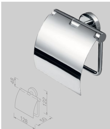
Toiletrolhouder met klep Toilet roll holder with cover 916508-02
