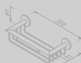
Douchemand 30 cm Shower basket 30 cm
