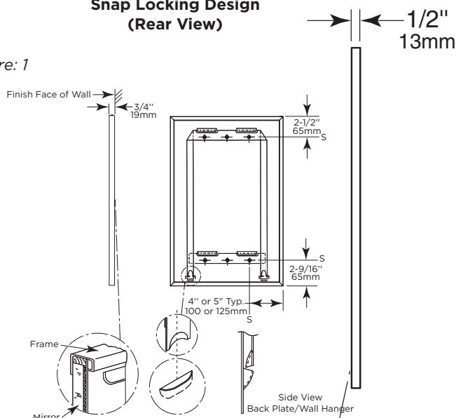
STANDARD B-290 SERIES MIRRORS
