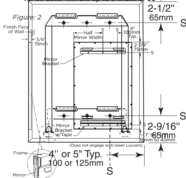
"2S" Tab Design (Rear View)
