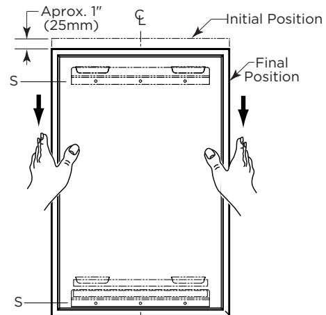
"2S" Tab Design- Up to 36" Width (Front View)
